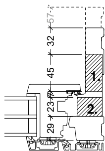
149mm + 174mm karm
